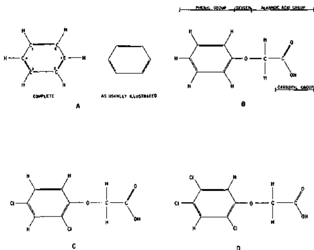
Figure 3. Construction of 2,4-D and 2,4,5-T. A, organic structure of the benzene ring. B, the general phenoxy model. C, 2,4-dichlorophenoxyacetic acid (2,4-D). D, 2,4,5-trichlorophenoxyacetic acid (2,4,5-T).
