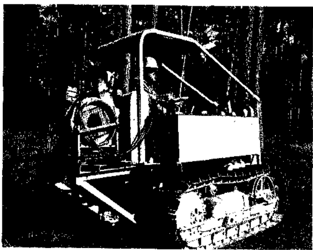
U. S. Forest Service photo. Figure 9. The tractor-mounted mist blower has become a popular silvicultural tool in the southeast. It will travel almost anywhere and can effectively treat trees 30 to 40 feet high.
