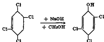
1,2,4,5-tetrachlorobenzene 2,4,5-trichlorophenol Alkaline hydrolysis of 1,2,4,5-tetrachlorobenzene into 2,4,5-trichlorophenol.
