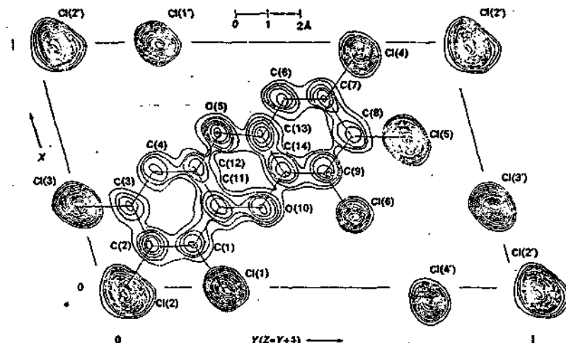
Fig. 4. Electron density in the (034) plane containing the molecule. Contours are at 1 \text{ e} \cdot \text{Å}^{-3} starting at 2 \text{ e} \cdot \text{Å}^{-3} . The x marks are projections onto (034) from the electron density maxima, which in most cases are a short distance from (034).
