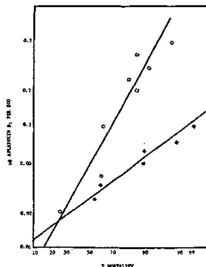
Fig. 1—Toxicity of aflatoxin B 1 in the chicken embryo: mortality at 21 days. LD 50 : yolk, 0.048 µg; air cell, 0.025 µg. Open squares: yolk injection. Closed squares: air cell injection.
