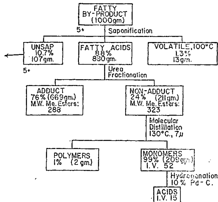
Fig. 1.—Fractionation of fatty acid by-product. (Numbers followed by + sign are toxicity scores; see footnote a, Table 5.)
