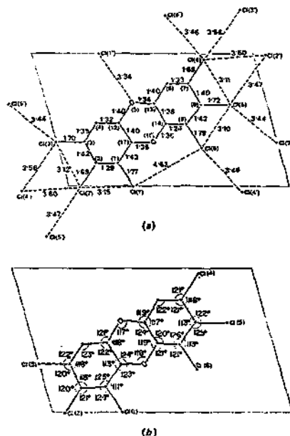
Fig. 3. (a) Interatomic distances. Primed atoms are on neighboring molecules in the same plane. \sigma_{C-C}=0.025 Å; \sigma_{C-Cl}=0.019 Å; \sigma_{C-O}=0.022 Å. View corresponds to Fig. 1. (b) Bond angles. \sigma=2.0^\circ .
