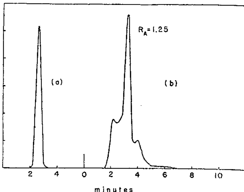
Fig. 2—Microcoulometric gas chromatograms of (a) aldrin standard (1 µg), and (b) alumina fraction 2 from USP cottonseed oil without added toxic fat.
