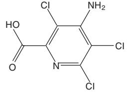
FIGURE 2-2 Chemical structures and CAS numbers for specific chemicals of interest.
